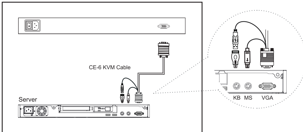
Figure 9. Example of connecting CE-6 Combo 4-in-1 KVM cable to server via PS/2 interface
