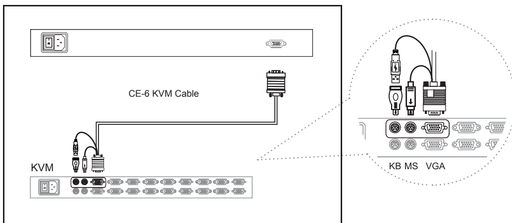
Figure 10. Example of connecting CE-6 Combo 4-in-1 KVM cable to KVM via PS/2 interface
