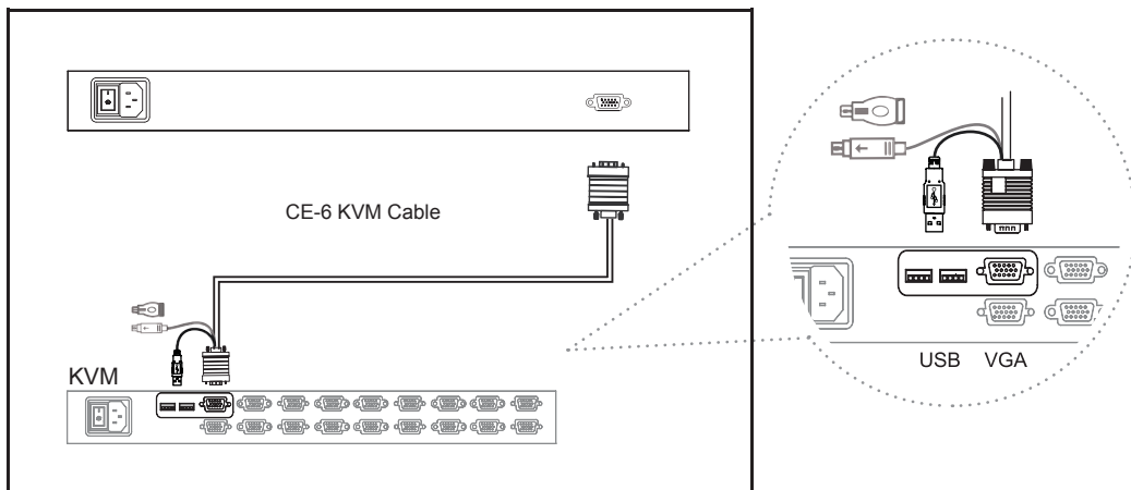
Figure 12. Example of connecting CE-6 Combo 4-in-1 KVM cable to KVM via USB interface
