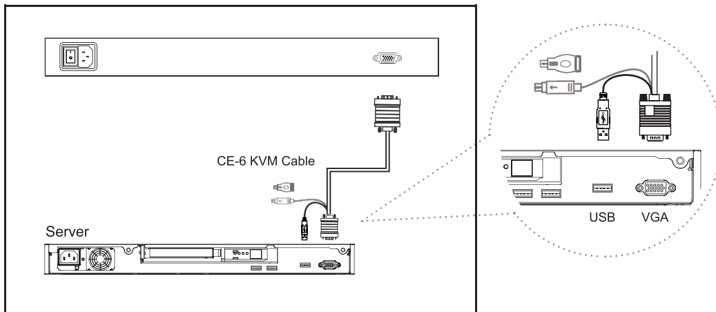
Figure 11. Example of connecting CE-6 Combo 4-in-1 KVM cable to server via USB interface
