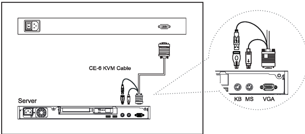
Figure 9. Example of connecting KVMCE-6 Combo 4-in-1 KVM cable to server via PS/2 interface
