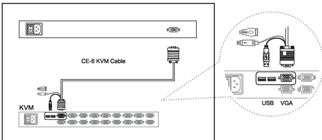
Figure 12. Example of connecting KVMCE-6 Combo 4-in-1 KVM cable to KVM via USB interface
