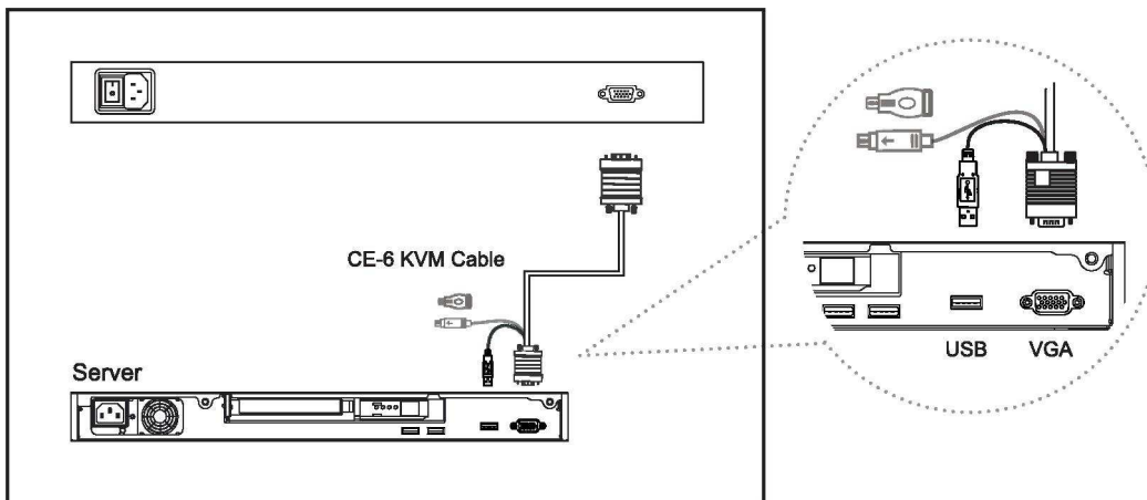
Figure 11. Example of connecting KVMCE-6 Combo 4-in-1 KVM cable to server via USB interface
