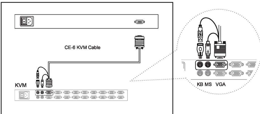
Figure 10. Example of connecting KVMCE-6 Combo 4-in-1 KVM cable to KVM via PS/2 interface
