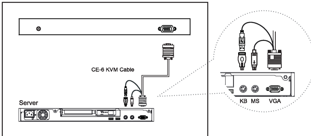
Figure 13. Example of connecting KVMCE-6 Combo 4-in-1 KVM cable to server via PS/2 interface
