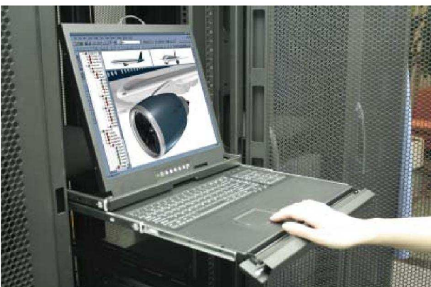
Figure 4. Operating the LCD keyboard drawer.
