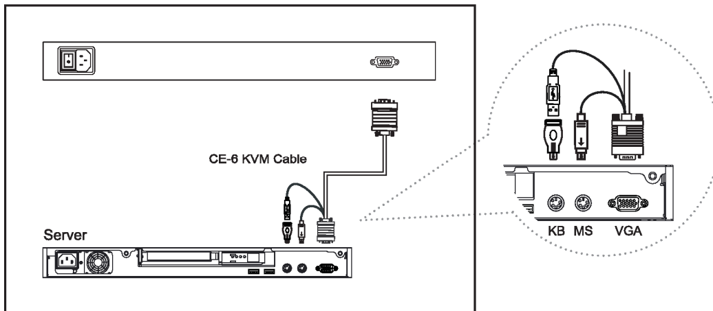
Figure 9. Example of connecting KVMCE-6 Combo 4-in-1 KVM cable to server via PS/2 interface
