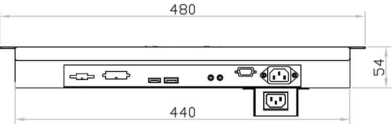
Bottom View
